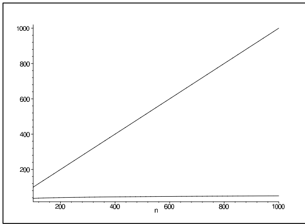
Fig. 2. signature retrieval cost (bottom) compared with full database retrieval cost (top) with a single record mismatch versus database size: Q = 16 , b = 16
